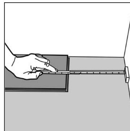
Figure 49 Last plank, first row
