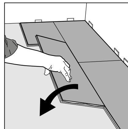
Figure 17 Second plank, second row
