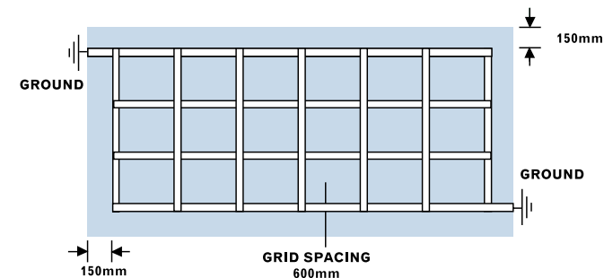
Figure 2 Earth strip layout
